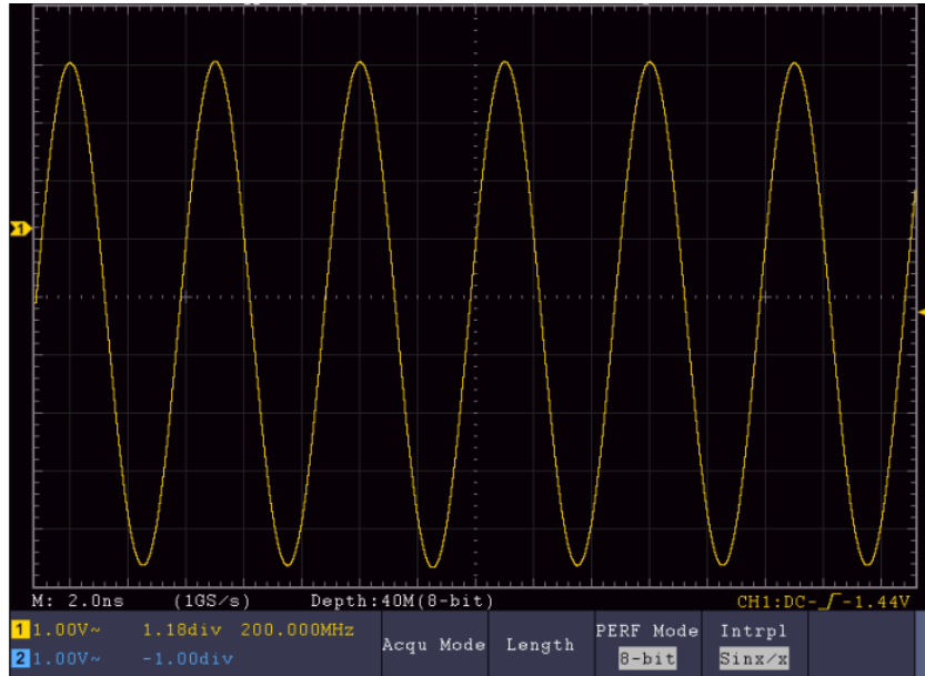
Sine(x)/x interpolation
